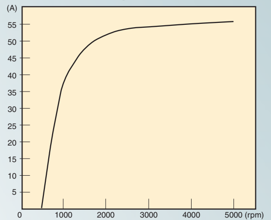
Alternator Output
